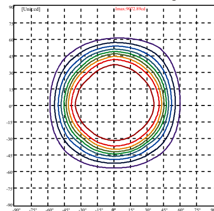
ISO Illuminance Diagram
