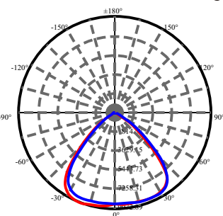
Illuminance Distribution Diagram
